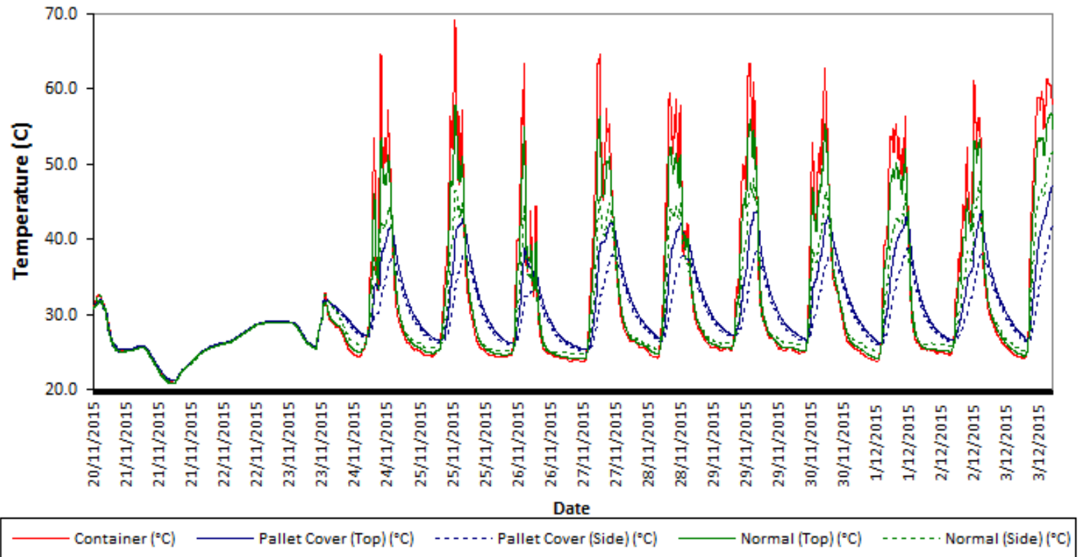
Comparison of Temperature with and without Pallet Cover
